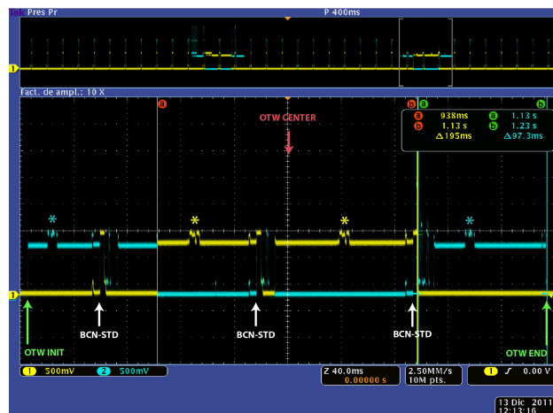
Fig. 12: Prioritized scheduling.
