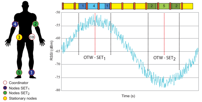
Fig. 7: OTW and transmission schedules. Transmissions from nodes 4 and 5 have higher priority.
