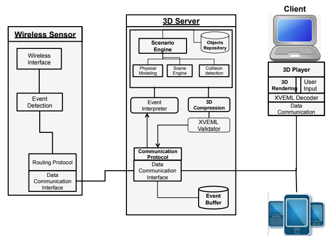
Figure 1. 3D Virtual Disaster Management System Architecture
