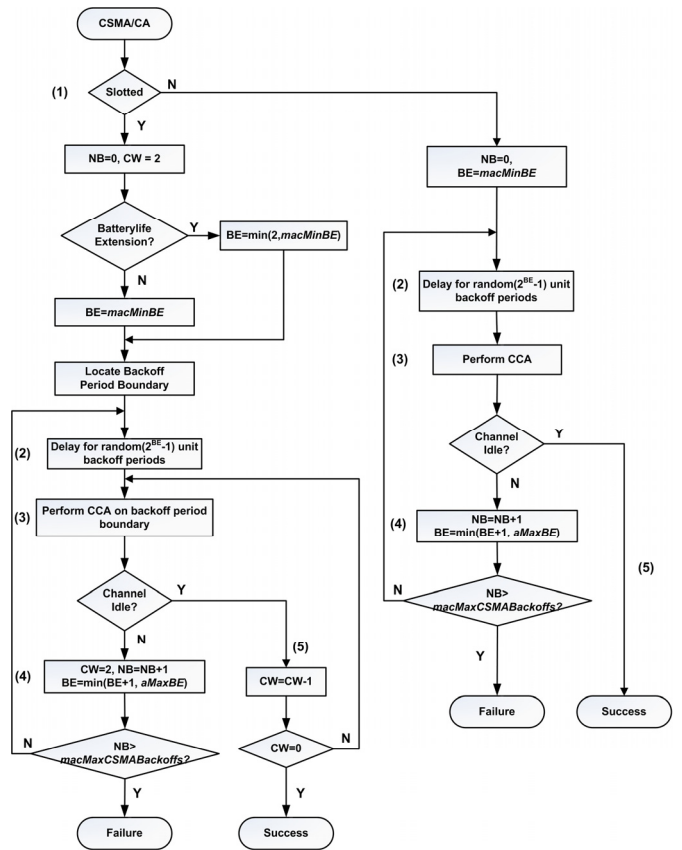
Fig. 14. The CSMA/CA Mechanism
